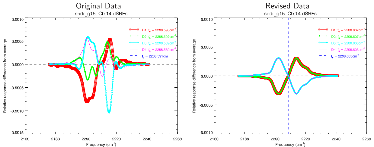
Figure 3.5: Difference of the GOES-P(15) Sounder individual detector SRFs from the average SRF for channel 14. The vertical dashed line indicates f_0 . (Left Panel) Original SRF data showing the differences between detectors. (Right Panel) Revised SRF data still showing differences.
