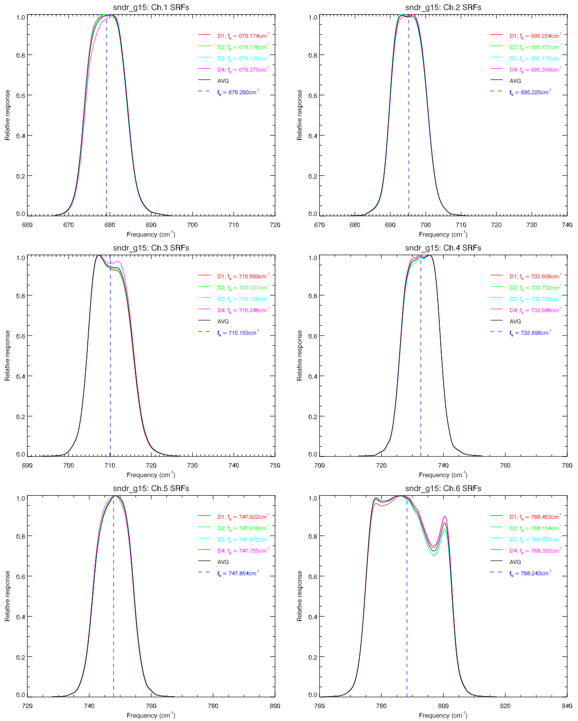
Figure B.1: GOES-P(15) Sounder SRF for channels 1 to 6.
