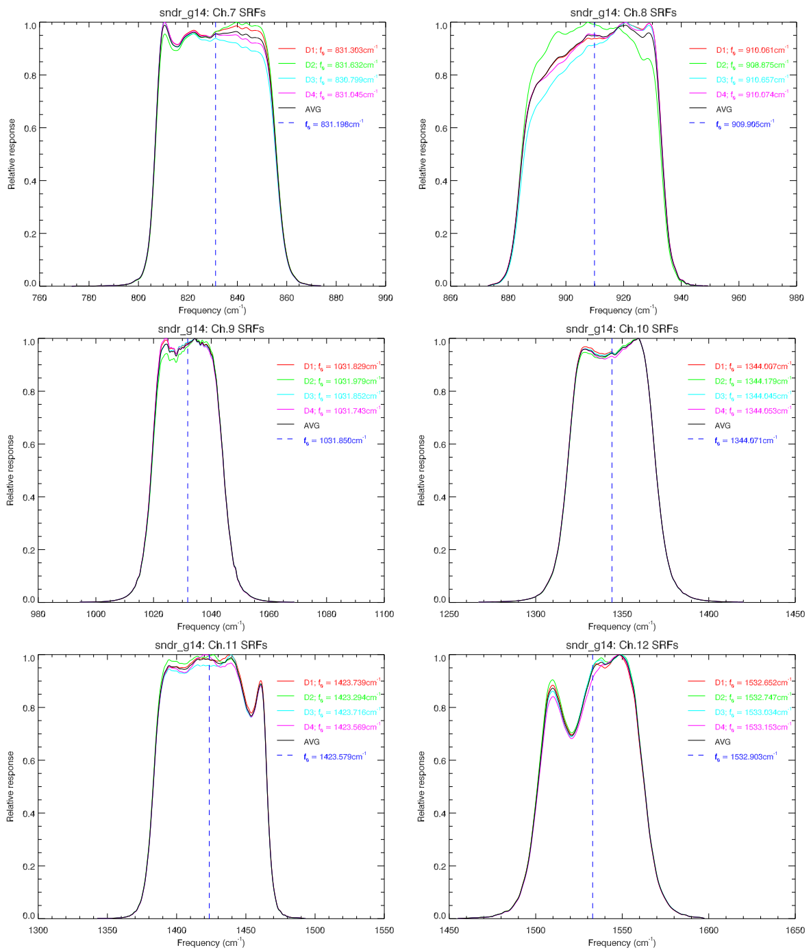
Figure A.2: GOES-O(14) Sounder SRF for channels 7 to 12.
