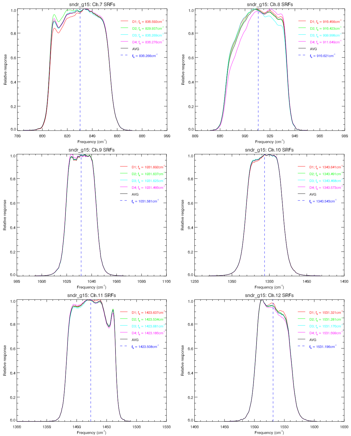
Figure B.2: GOES-P(15) Sounder SRF for channels 7 to 12.
