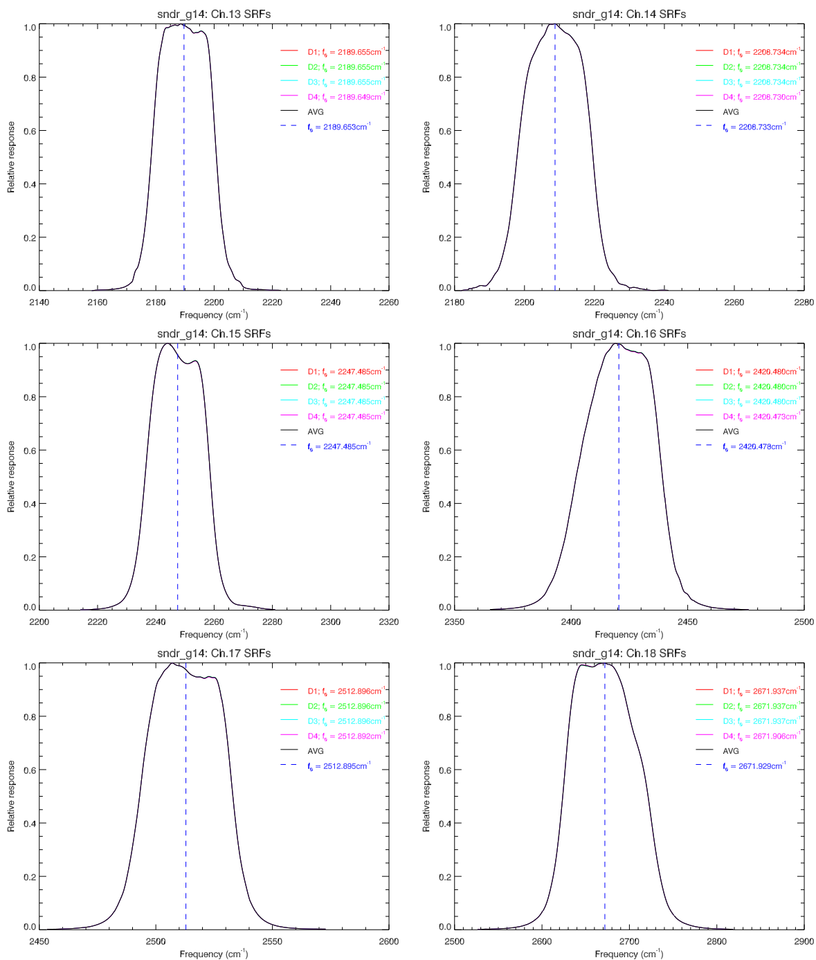
Figure A.3: GOES-O(14) Sounder SRF for channels 13 to 18.
