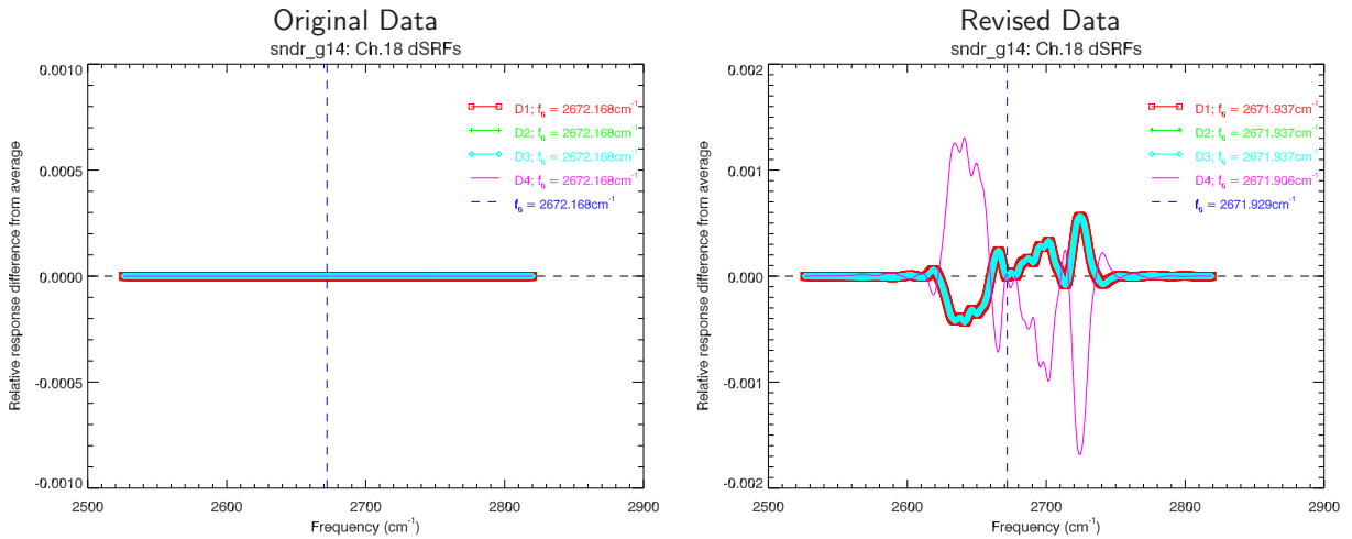
Figure 2.12: Difference of the GOES-O(14) Sounder individual detector SRFs from the average SRF for channel 18. The vertical dashed line indicates f_0 . (Left Panel) Original SRF data showing no differences between detectors. (Right Panel) Revised SRF data now showing differences due to detector #4.
