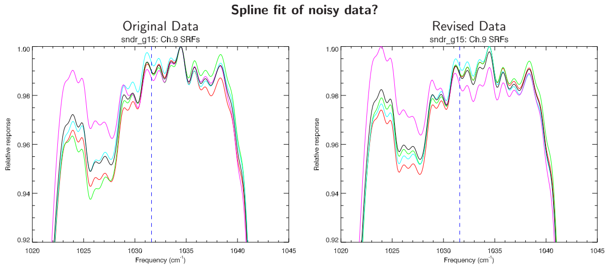
Figure 3.1: Magnification of GOES-P(15) Sounder individual detector and average SRFs for channel 9. The detector average SRF is plotted in black. The vertical dashed line indicates f_0 . (Left Panel) Original SRF data showing the anomaly. (Right Panel) Revised SRF data showing similar behaviour.
