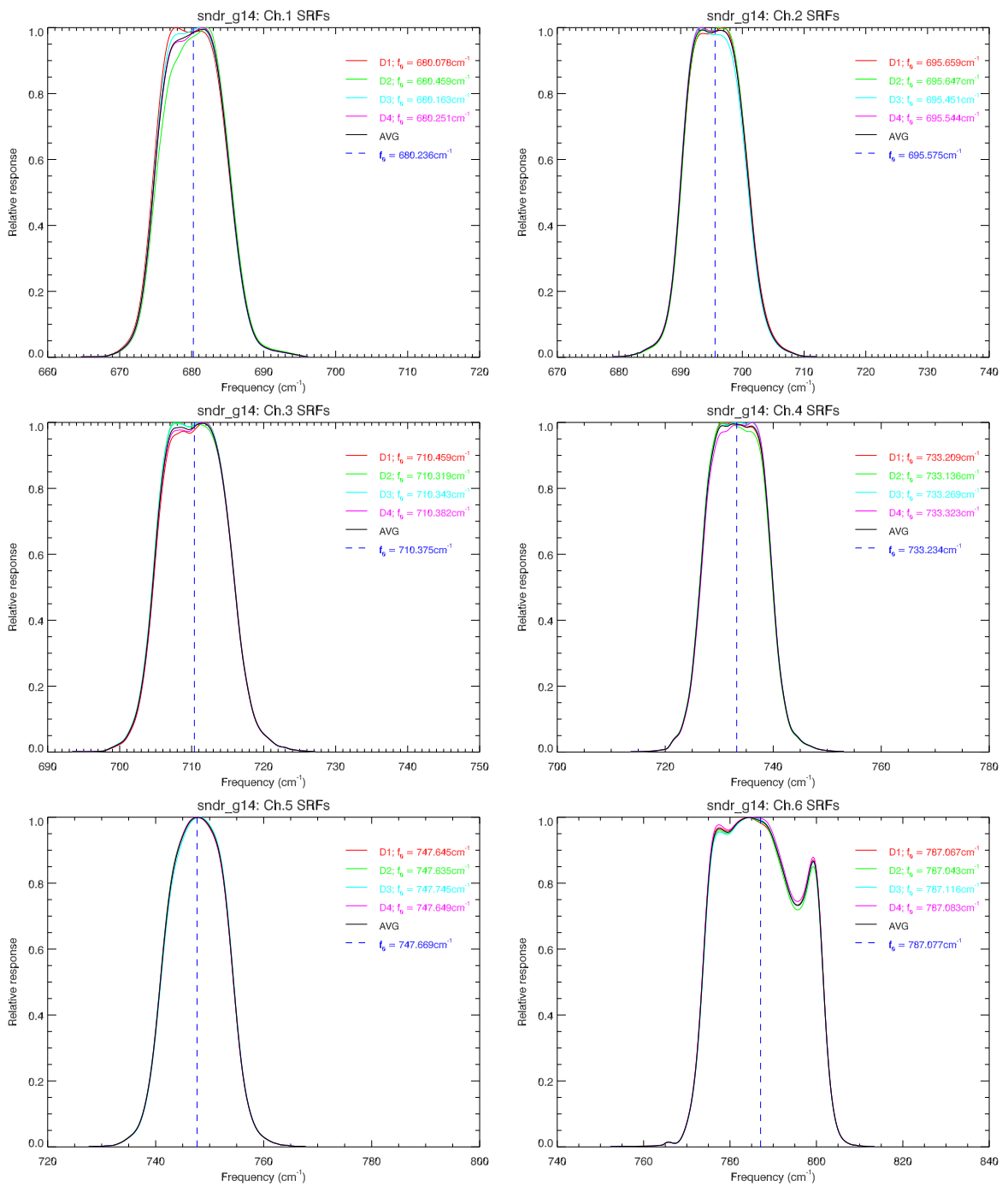
Figure A.1: GOES-O(14) Sounder SRF for channels 1 to 6.
