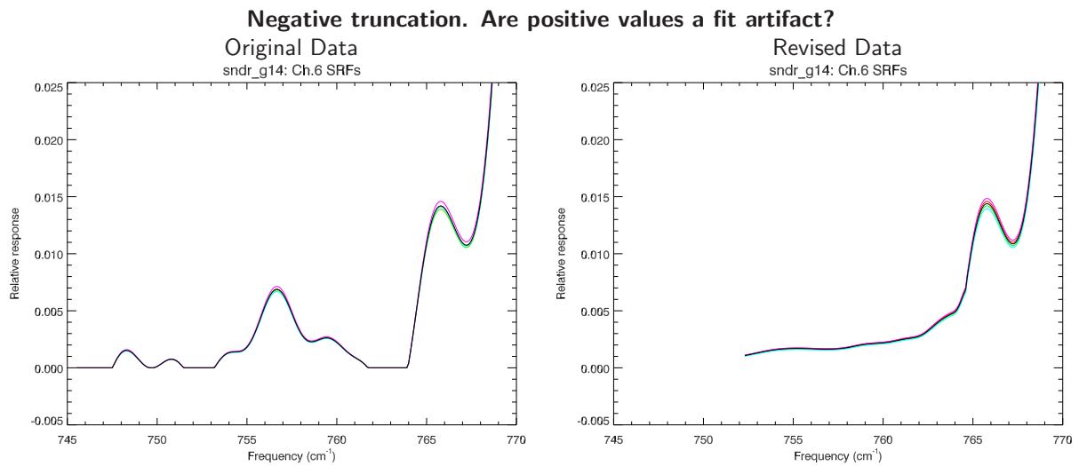
Figure 2.2: Magnification of GOES-O(14) Sounder individual detector and average SRFs for channel 6. The detector average SRF is plotted in black. (Left Panel) Original SRF data showing the anomaly. (Right Panel) Revised SRF data with no anomaly.
