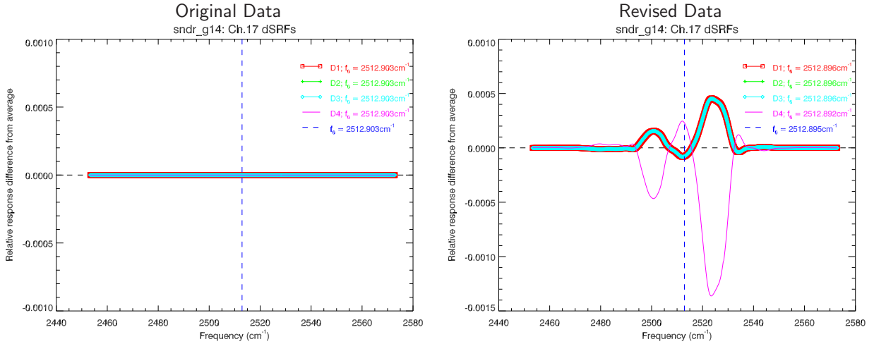
Figure 2.11: Difference of the GOES-O(14) Sounder individual detector SRFs from the average SRF for channel 17. The vertical dashed line indicates f_0 . (Left Panel) Original SRF data showing no differences between detectors. (Right Panel) Revised SRF data now showing differences due to detector #4.
