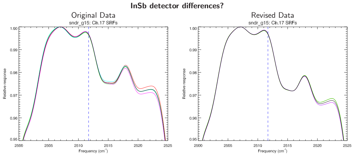
Figure 3.8: Magnification of GOES-P(15) Sounder individual detector and average SRFs for channel 17. The detector average SRF is plotted in black. The vertical dashed line indicates f_0 . (Left Panel) Original SRF data showing the anomaly. (Right Panel) Revised SRF data still showing differences between detectors.
