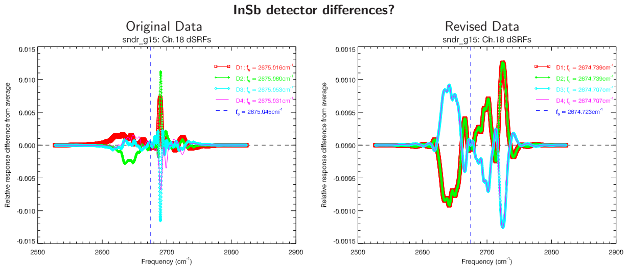
Figure 3.11: Difference of the GOES-P(15) Sounder individual detector SRFs from the average SRF for channel 18. The vertical dashed line indicates f_0 . (Left Panel) Original SRF data showing the differences between detectors. (Right Panel) Revised SRF data still showing differences.
