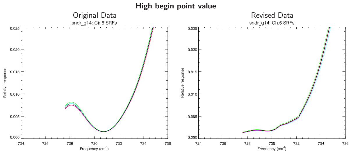
Figure 2.1: Magnification of GOES-O(14) Sounder individual detector and average SRFs for channel 5. The detector average SRF is plotted in black. (Left Panel) Original SRF data showing the anomaly. (Right Panel) Revised SRF data with no anomaly.
