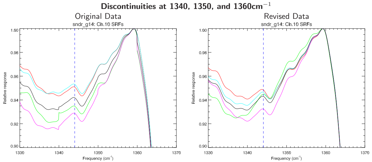
Figure 2.4: Magnification of GOES-O(14) Sounder individual detector and average SRFs for channel 10. The detector average SRF is plotted in black. The vertical dashed line indicates f_0 . (Left Panel) Original SRF data showing the anomaly. (Right Panel) Revised SRF data with no anomaly.
