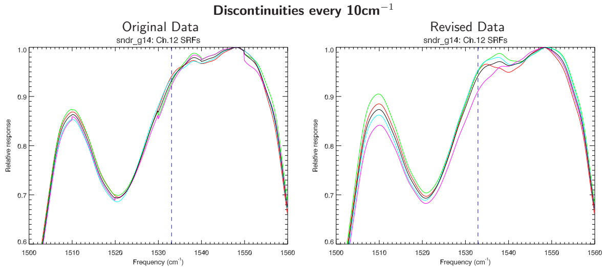
Figure 2.6: Magnification of GOES-O(14) Sounder individual detector and average SRFs for channel 12. The detector average SRF is plotted in black. The vertical dashed line indicates f_0 . (Left Panel) Original SRF data showing the anomaly. (Right Panel) Revised SRF data with no anomaly.
