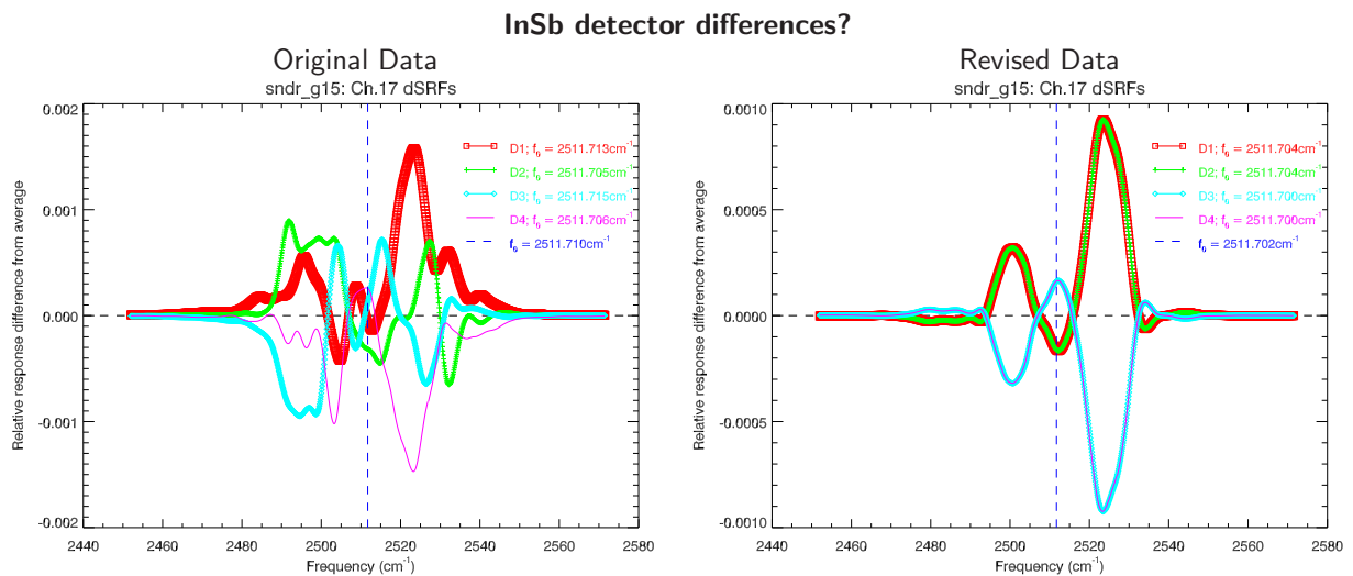
Figure 3.9: Difference of the GOES-P(15) Sounder individual detector SRFs from the average SRF for channel 17. The vertical dashed line indicates f_0 . (Left Panel) Original SRF data showing the differences between detectors. (Right Panel) Revised SRF data still showing differences.
