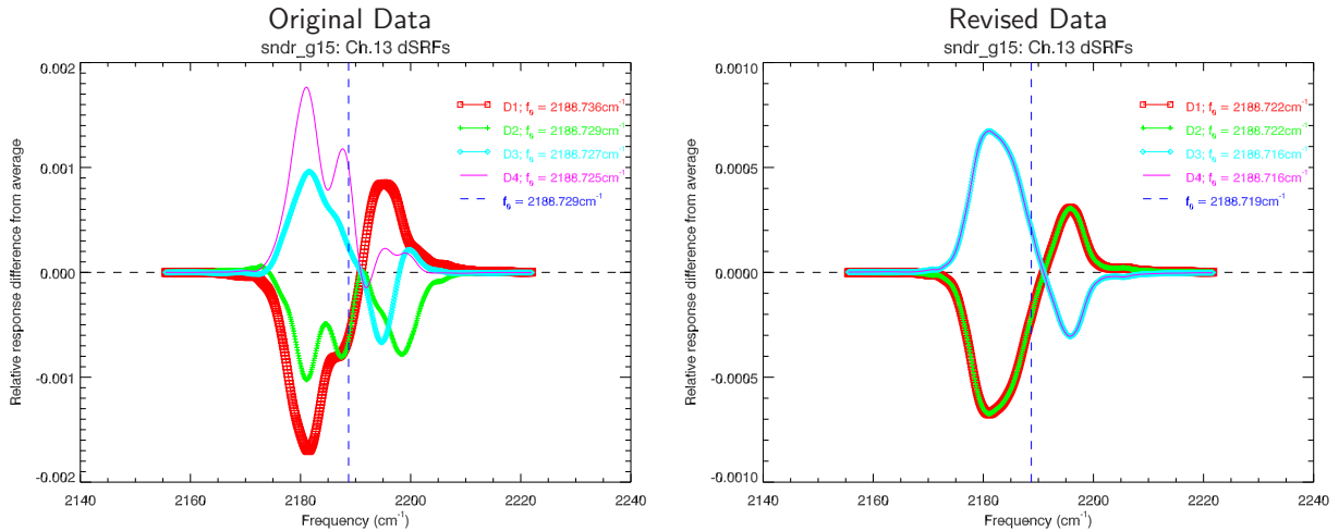
Figure 3.4: Difference of the GOES-P(15) Sounder individual detector SRFs from the average SRF for channel 13. The vertical dashed line indicates f_0 . (Left Panel) Original SRF data showing the differences between detectors. (Right Panel) Revised SRF data still showing differences.
