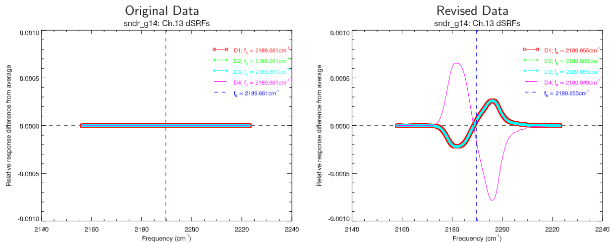
Figure 2.7: Difference of the GOES-O(14) Sounder individual detector SRFs from the average SRF for channel 13. The vertical dashed line indicates f_0 . (Left Panel) Original SRF data showing no differences between detectors. (Right Panel) Revised SRF data now showing differences due to detector #4.
