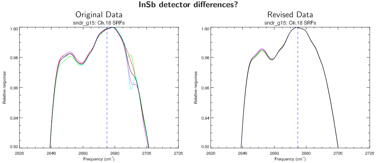
Figure 3.10: Magnification of GOES-P(15) Sounder individual detector and average SRFs for channel 18. The detector average SRF is plotted in black. The vertical dashed line indicates f_0 . (Left Panel) Original SRF data showing the anomaly. (Right Panel) Revised SRF data still showing differences between detectors.
