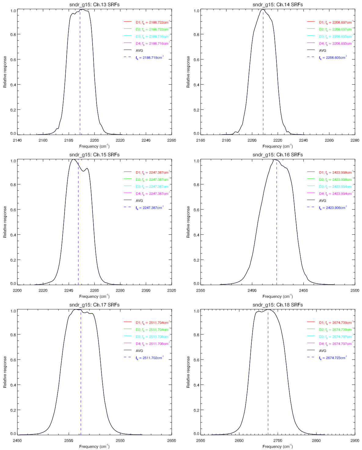
Figure B.3: GOES-P(15) Sounder SRF for channels 13 to 18.
