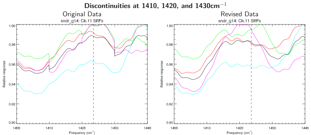
Figure 2.5: Magnification of GOES-O(14) Sounder individual detector and average SRFs for channel 11. The detector average SRF is plotted in black. The vertical dashed line indicates f_0 . (Left Panel) Original SRF data showing the anomaly. (Right Panel) Revised SRF data with no anomaly.
