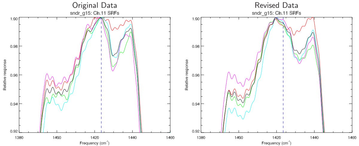
Figure 3.2: Magnification of GOES-P(15) Sounder individual detector and average SRFs for channel 11. The detector average SRF is plotted in black. The vertical dashed line indicates f_0 . (Left Panel) Original SRF data showing the anomaly. (Right Panel) Revised SRF data showing similar behaviour.
