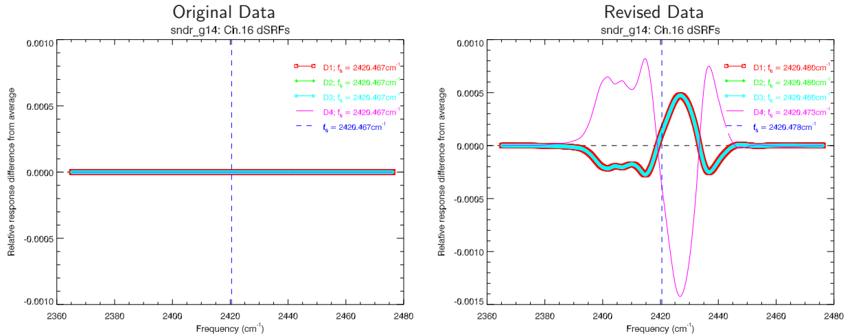
Figure 2.10: Difference of the GOES-O(14) Sounder individual detector SRFs from the average SRF for channel 16. The vertical dashed line indicates f_0 . (Left Panel) Original SRF data showing no differences between detectors. (Right Panel) Revised SRF data now showing differences due to detector #4.
