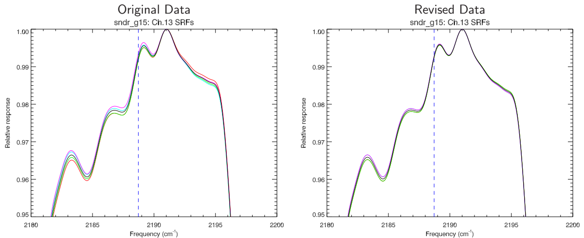
Figure 3.3: Magnification of GOES-P(15) Sounder individual detector and average SRFs for channel 13. The detector average SRF is plotted in black. The vertical dashed line indicates f_0 . (Left Panel) Original SRF data showing the anomaly. (Right Panel) Revised SRF data still showing differences between detectors.
