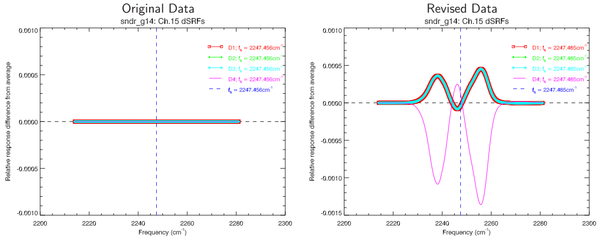
Figure 2.9: Difference of the GOES-O(14) Sounder individual detector SRFs from the average SRF for channel 15. The vertical dashed line indicates f_0 . (Left Panel) Original SRF data showing no differences between detectors. (Right Panel) Revised SRF data now showing differences due to detector #4.
