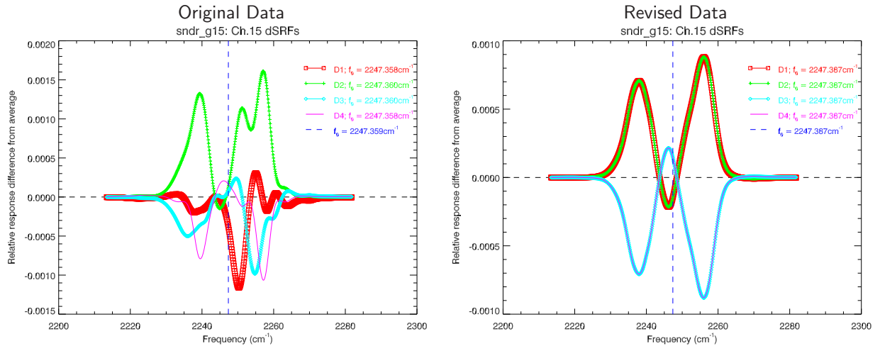
Figure 3.6: Difference of the GOES-P(15) Sounder individual detector SRFs from the average SRF for channel 15. The vertical dashed line indicates f_0 . (Left Panel) Original SRF data showing the differences between detectors. (Right Panel) Revised SRF data still showing differences.
