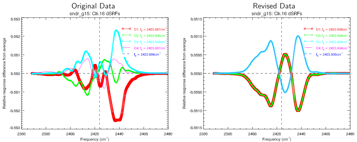
Figure 3.7: Difference of the GOES-P(15) Sounder individual detector SRFs from the average SRF for channel 16. The vertical dashed line indicates f_0 . (Left Panel) Original SRF data showing the differences between detectors. (Right Panel) Revised SRF data still showing differences.
