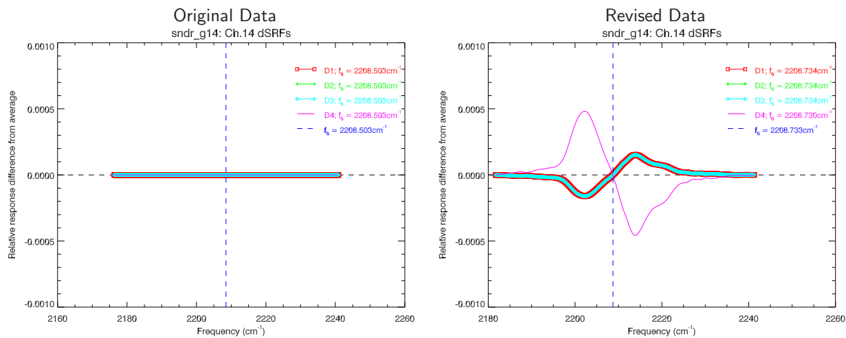
Figure 2.8: Difference of the GOES-O(14) Sounder individual detector SRFs from the average SRF for channel 14. The vertical dashed line indicates f_0 . (Left Panel) Original SRF data showing no differences between detectors. (Right Panel) Revised SRF data now showing differences due to detector #4.
