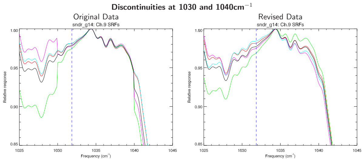
Figure 2.3: Magnification of GOES-O(14) Sounder individual detector and average SRFs for channel 9. The detector average SRF is plotted in black. The vertical dashed line indicates f_0 . (Left Panel) Original SRF data showing the anomaly. (Right Panel) Revised SRF data with no anomaly.
