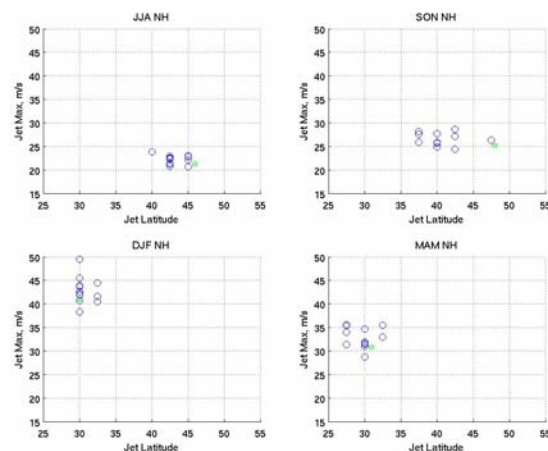
Fig.1 Seasonal mean zonal mean zonal wind jet maximum strength and latitude of the jet maxima for the ECMWF reanalysis (1989-2001, blue circles) and the Nature Run (green star), northern hemisphere. (by N. Prive.)
