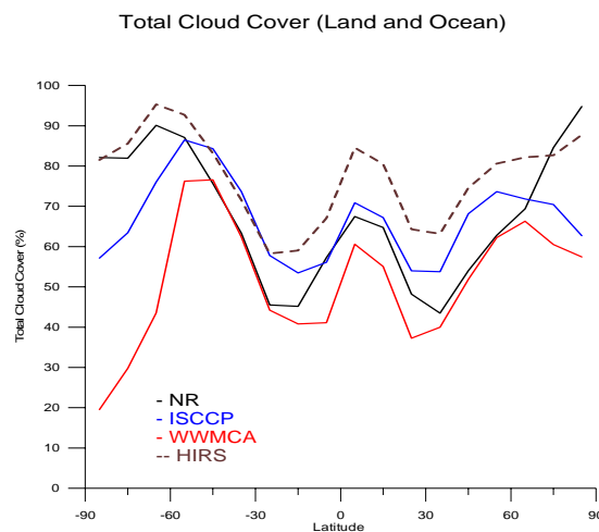
Fig.2 Zonal mean total cloud cover for AUGUST 2005. IT511 NR is compared with ISCCP monthly cloud climatologies, MODIS based cloud climatology, UW/HIRS based climatology, WWMCA (Nephanalyses) (by S. Greco.)
