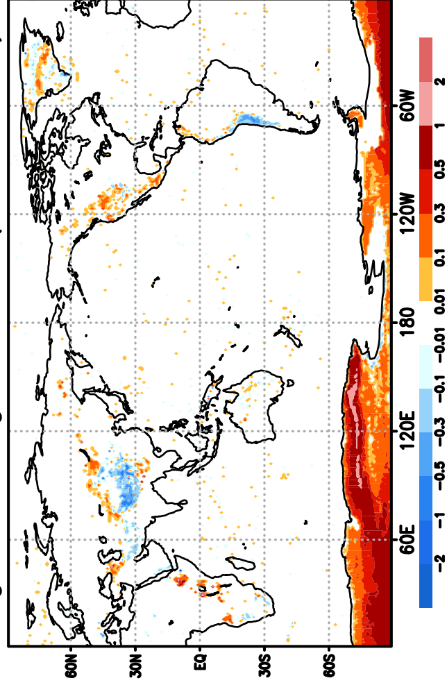
gfsv16bm - gfsv16bm2 (0.006,0.000)
