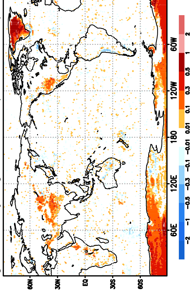
gfs16vti80j1 - gfsv16bm2 (0.007,0.000)
