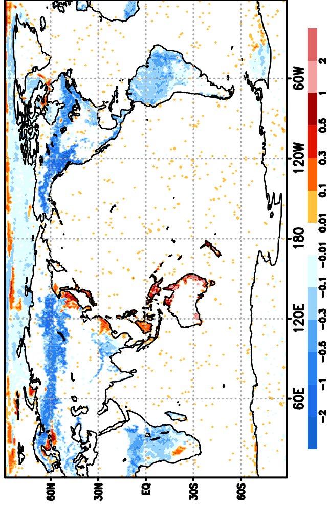
gfs16vti80j1 - gfsv16bm2 (-0.03, -0.01)
