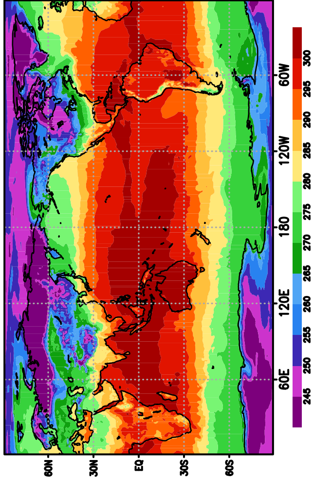
gfsv16bm2 TMPsfc FH=18
