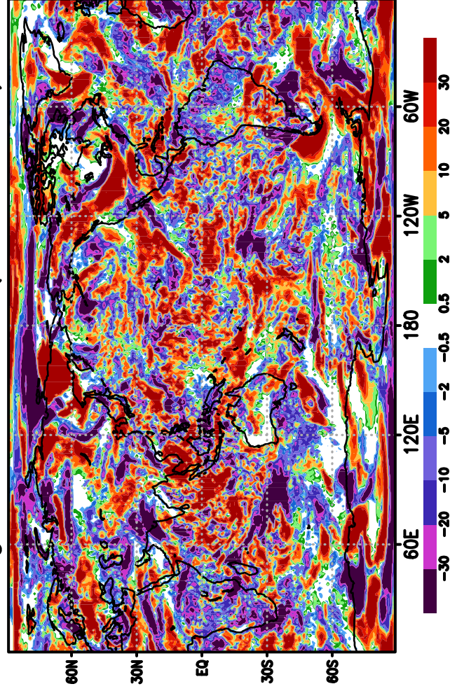
fv3gradr3 TCDCcIm (1.484,1.722)
