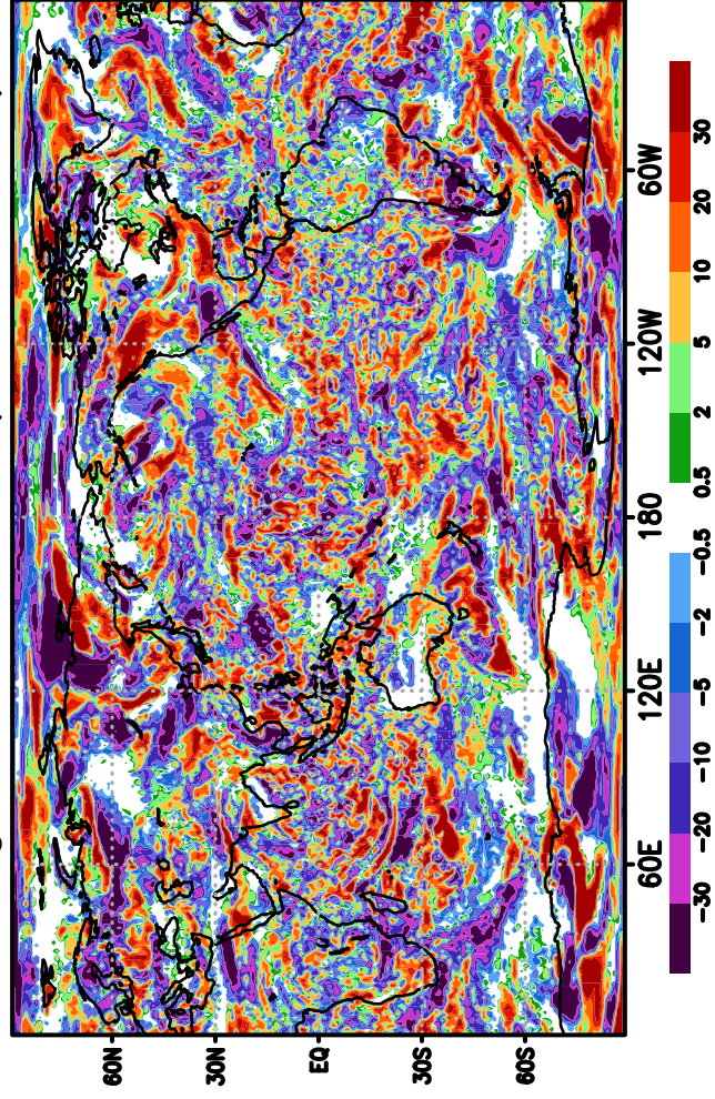
fv3gradr2 TCDCcIm (-0.64,-0.58)
