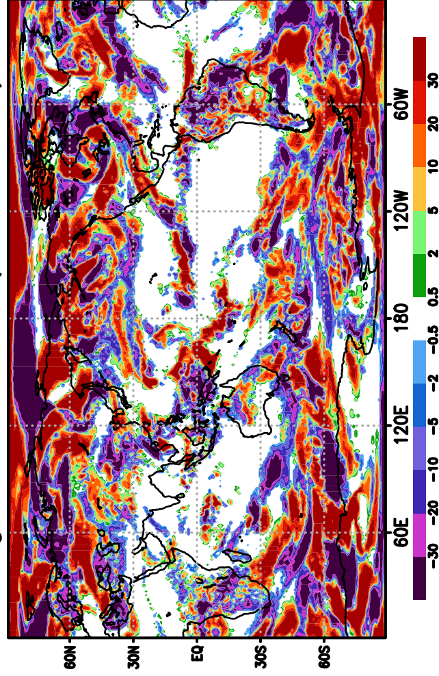
fv3gradr3 TCDCmcl (0.415,0.054)
