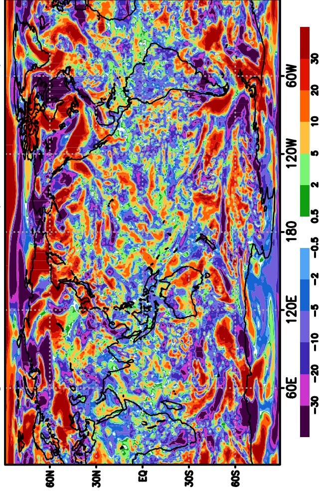
fv3gradr3 dlwrfsfc (0.216,-0.50)
