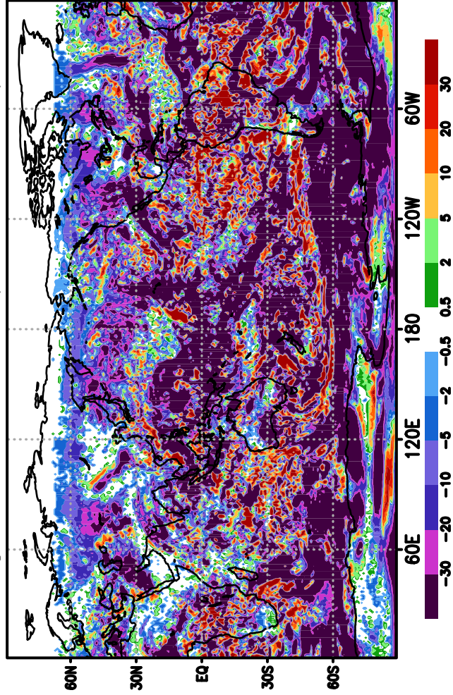
fv3gradr3 dswrfsfc (-23.6,-24.3)
