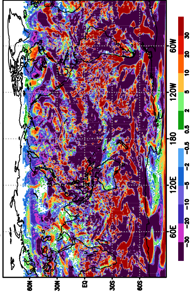
fv3gradr3 dswrfsfc (-21.8,-22.1)
