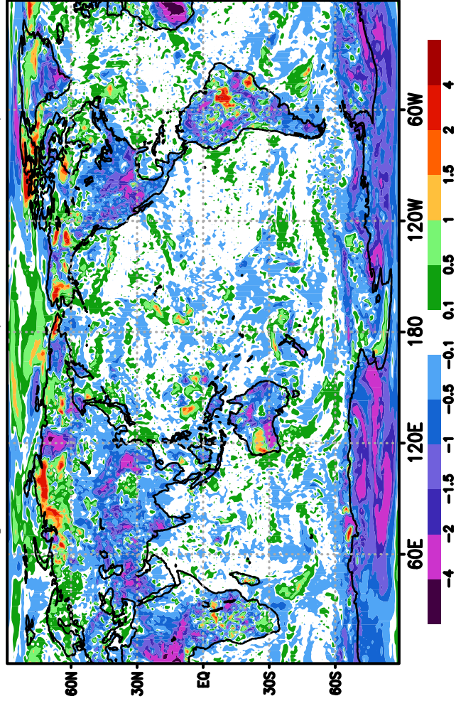
fv3gradr3 T2m ( -0.19, -0.17 )
