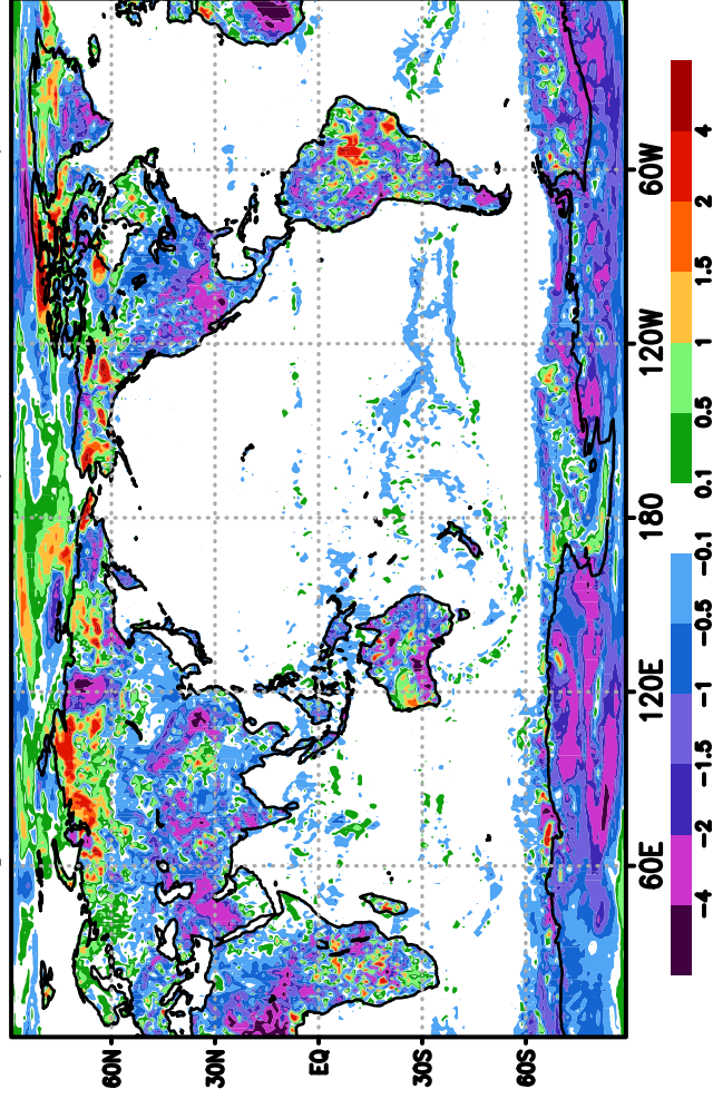
fv3gradr3 TMPsfc ( -0.21, -0.20 )
