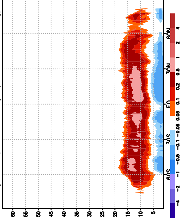
fv3gfsd temperature change (K, shal cnv heating)
