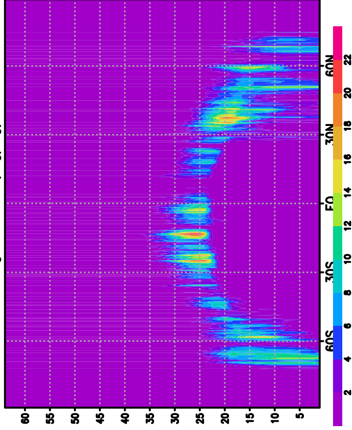
fv3gfsd snow (mg/kg)
