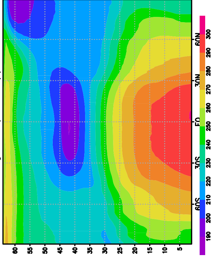
fv3gfsd temperature (k)
