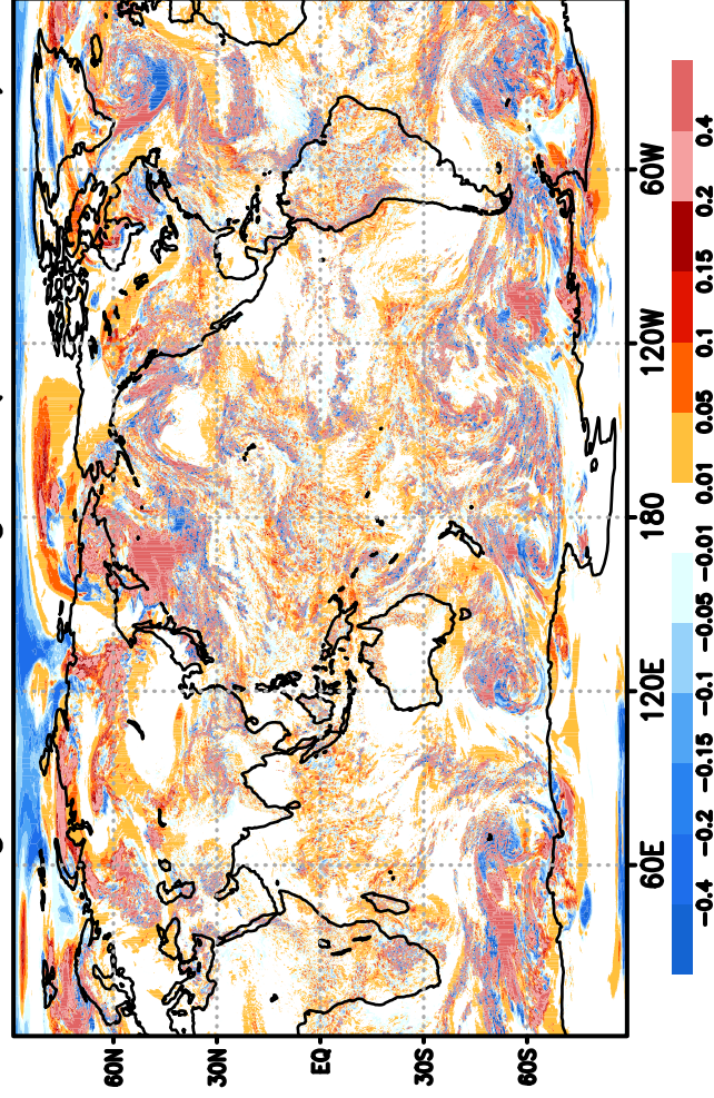
fv3gfdlradd-fv3gfsd (0.017,0.004)
