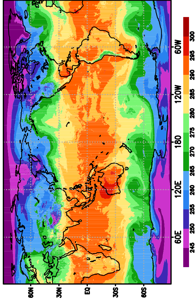
fv3gfsd TMP (279.0,288.9) F24H
