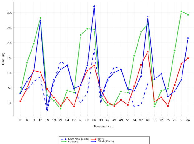
Mean PBL Height Error (August 2018) WEST
