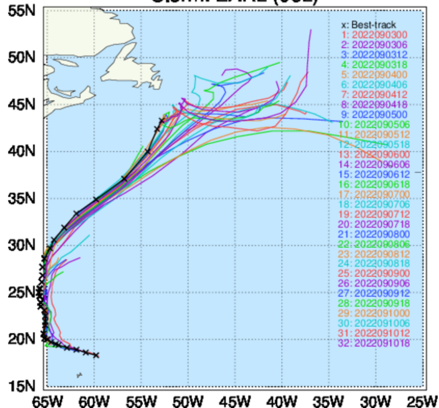
CH23 TC Tracks Storm: EARL (06L)
